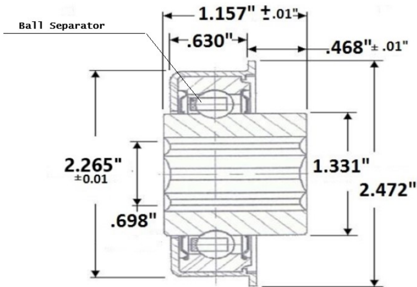
6205-2RS Core Bearing 1500 lb Load Rating
